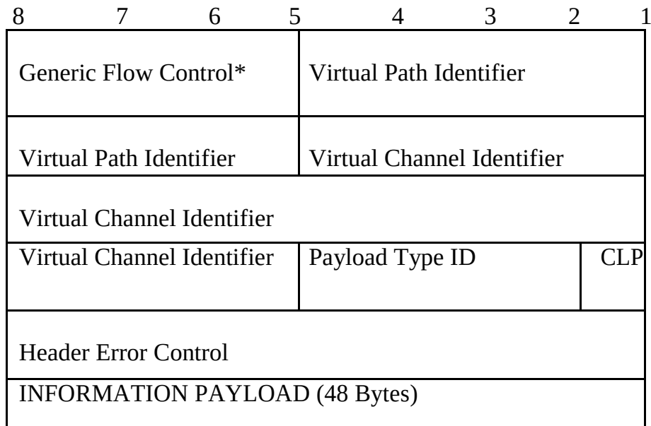
Figure 3: User–Network Interface
